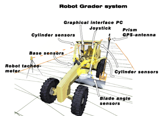
Figure. 2: Robot grader. A new 3-D blade control system principle for road grader.
