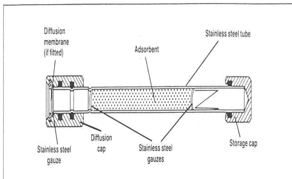
Figure 1. Diagram of a BTEX sampler fitted with a diffusion cap as worn by each participant in the pilot trial.
