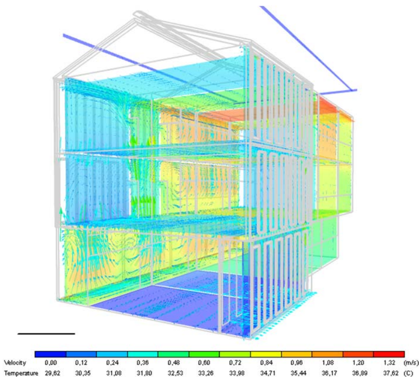
Fig. 2 CFD – thermal simulation on July 21 12:00 h in the classroom UPC Building , Girardot.
