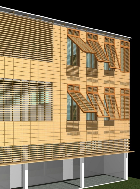
Fig. 3 UPC Classroom Building Rendering with bamboo guadua ventilated envelope
