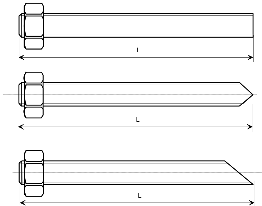
Different shapes of threaded rod ends : flat end, tow sides and one side 45° chamfer
