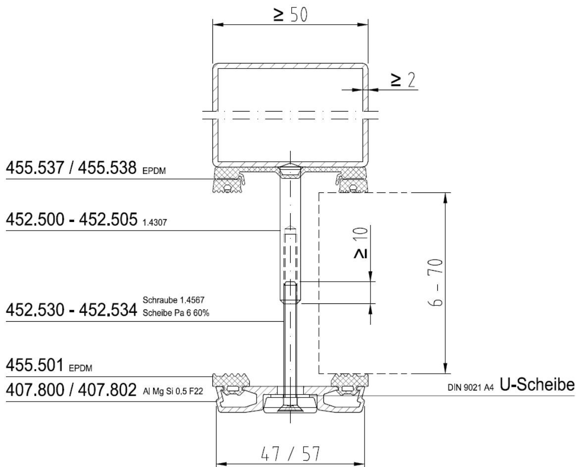
Figure 1 Profile JANSEN VISS Basic with welded bolt
