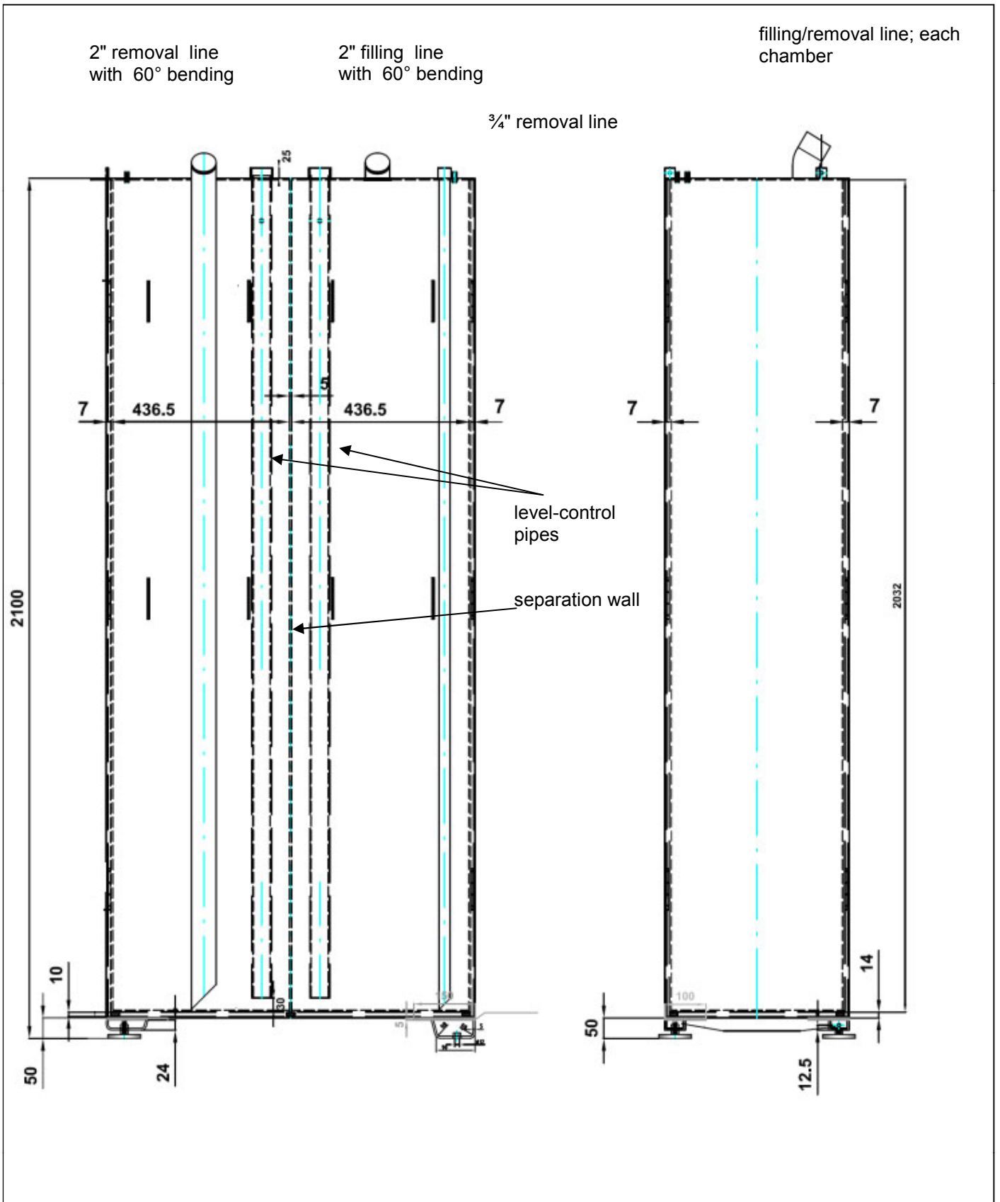
Double chamber oil storage tank for non-used and used lubricants
