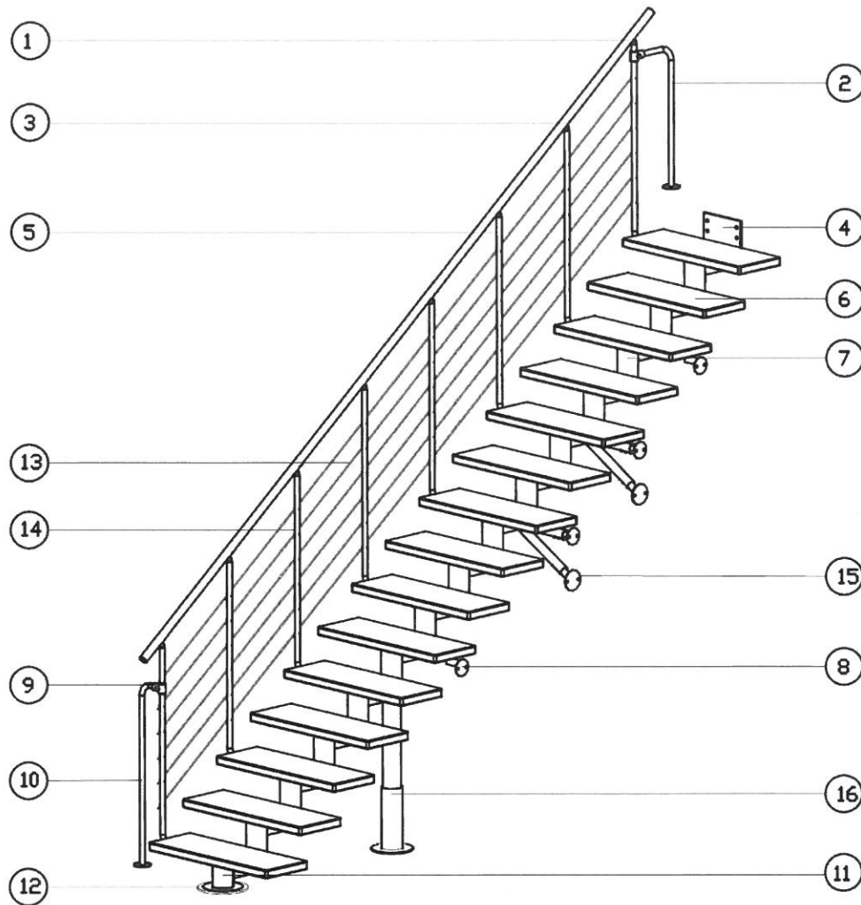
Components of the modular stairs type ATRIUM SEGMENT
