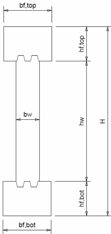
INOPANNE I-Joist with rectangular shaped bottom flange
