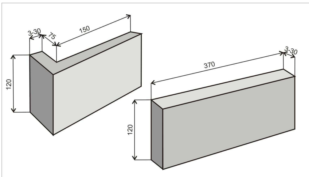
Fig. A1. Diagrams and dimensions of ALTAMIRA elements
