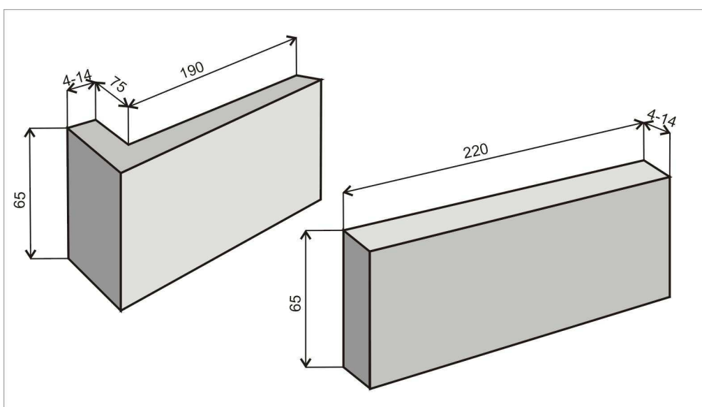
Fig. A2. Diagrams and dimensions of AMSTERDAM elements
