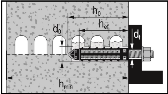
Figure A1: Hollow and solid brick with HAS-U-... and sieve sleeve HIT-SC (see Table B5)
