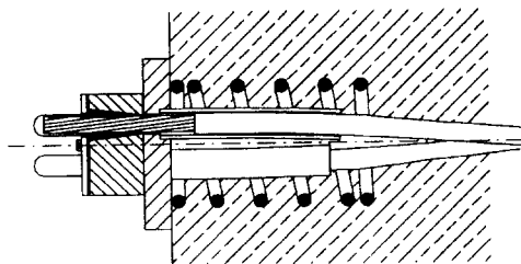
Stressing anchor MER6
