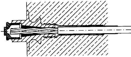
Stressing anchor SK6
