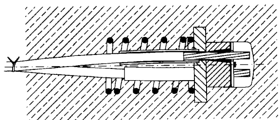
Fixed anchor MEF6
