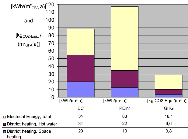
Figure 8: Site energy consumption (EC), non-renewable primary energy consumption (PEI nr ) and greenhouse gas emissions (GHG) for space heating (not standardized), hot water and electrical appliances per gross floor area (GFA) and year. Medium values of the period 09.2005 - 08.2007.
