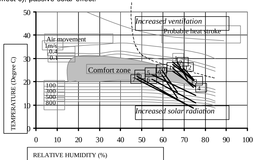
Figure 1 Olgyay's Bioclimatic chart applied to moderate climate of southeast Queensland, Australia
