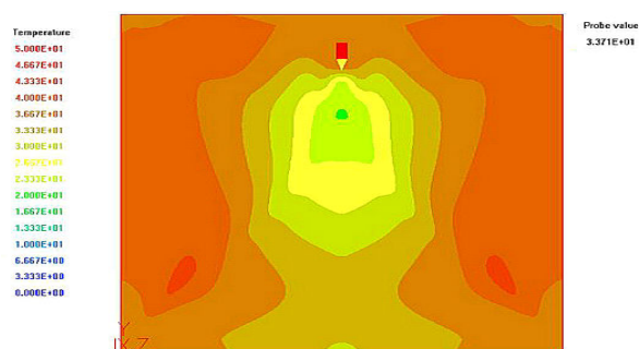
Figure 5. Temperature variation across the UTC under forced ventilation
