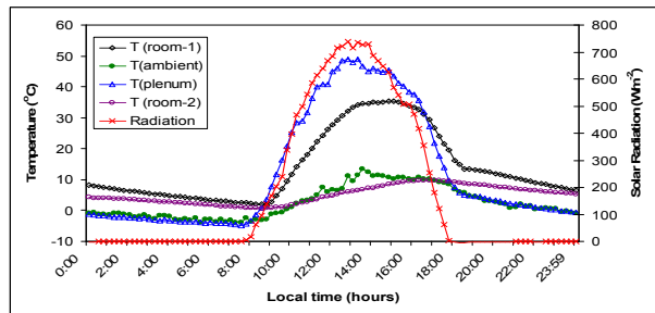
Figure 6. Variation of room and ambient temperatures and solar radiation with UTC and without UTC.
