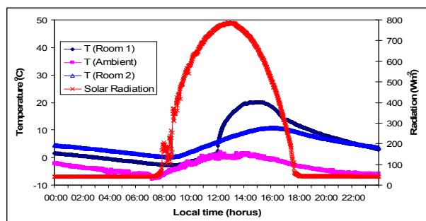
Figure 7. Variation of room temperatures, ambient temperatures and solar radiation in PVT hybrid air heating system and without UTC.
