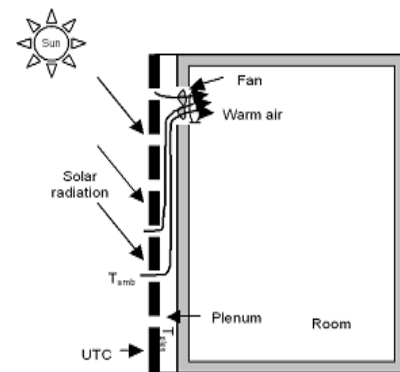
Figure 2. Schematic of UTC air heating system in KIER
