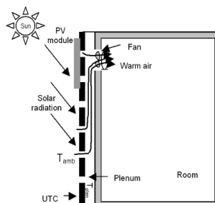
Figure 4. Schematic of PVT hybrid air heating system in KIER
