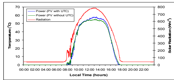
Figure 8. The electrical power outputs of PVT hybrid system and PV without UTC along with the incident global solar radiation in the plane of the PV modules.
