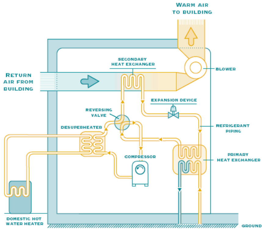
Figure 1: Typical Schematic for a Residential Water-to-Air Heat Pump System
