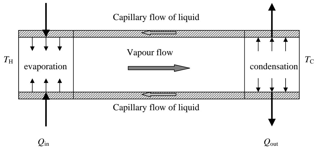
Figure 5: Schematic of a heat pipe.
