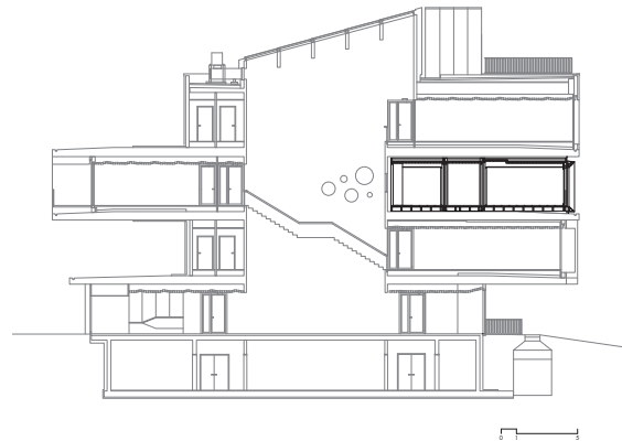
Figure 4. Section of NEST and UMAR
