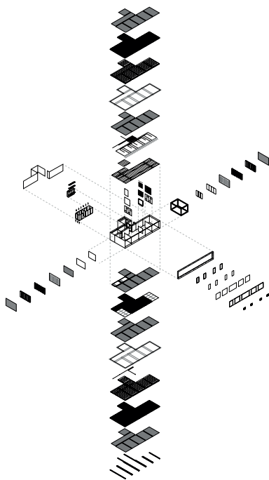
Figure 5. Axonometric representation of UMAR layers, hierarchy and assembly
