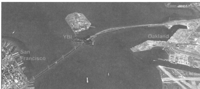
Fig. 3. Bay Bridge with New East crossing under construction
