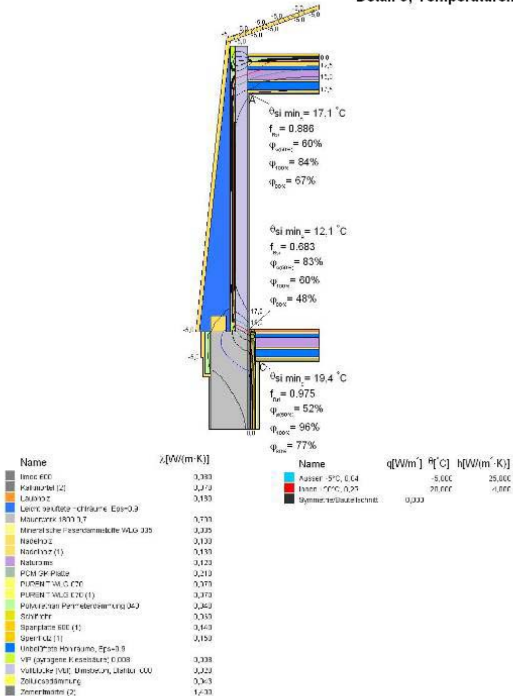
Detail 9; Temperaturen
