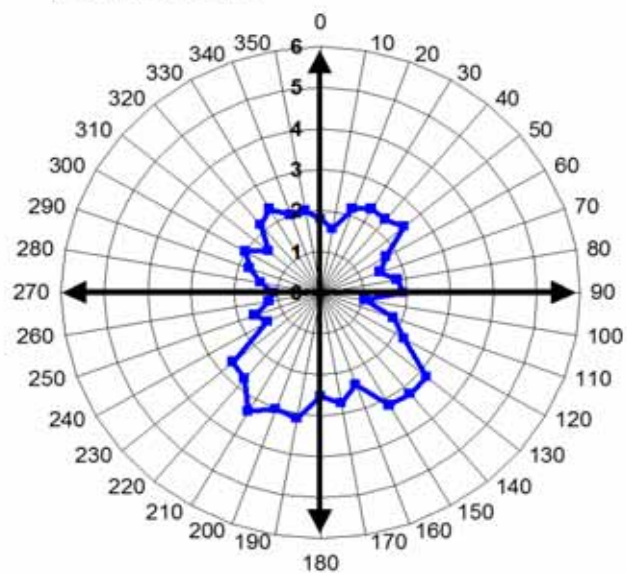
Anhang A 12: Polardiagramm Wind Apr 2010
