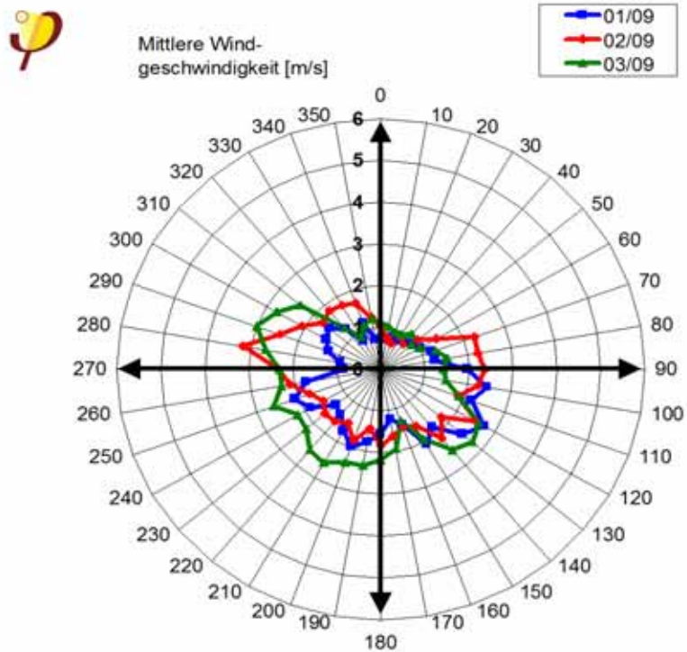
Anhang A 7: Polardiagramm Wind 1. Quartal 2009
