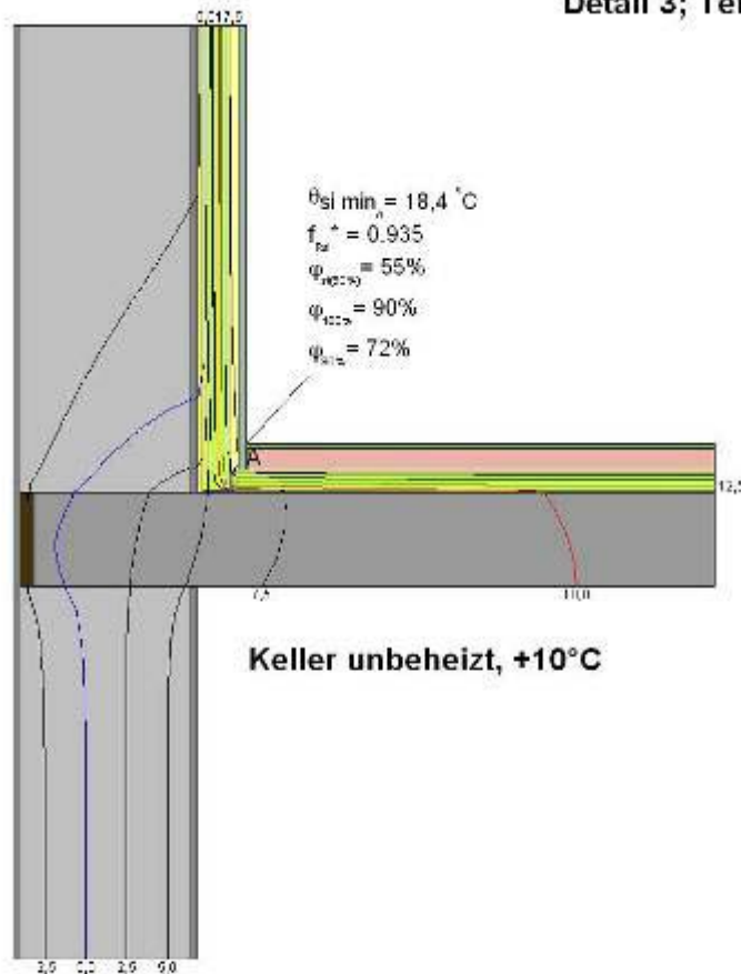
Detail 3; Temperaturen
