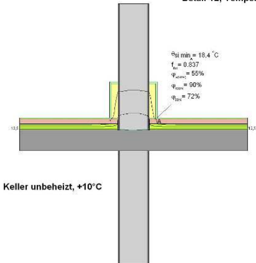
Detail 12; Temperaturen
