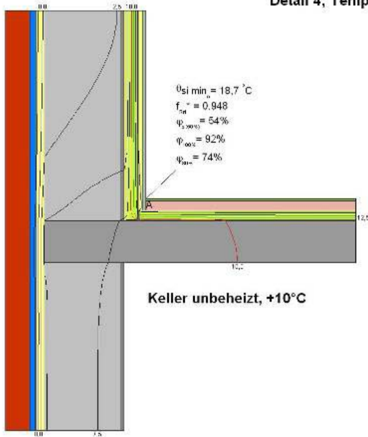
Detail 4; Temperaturen
