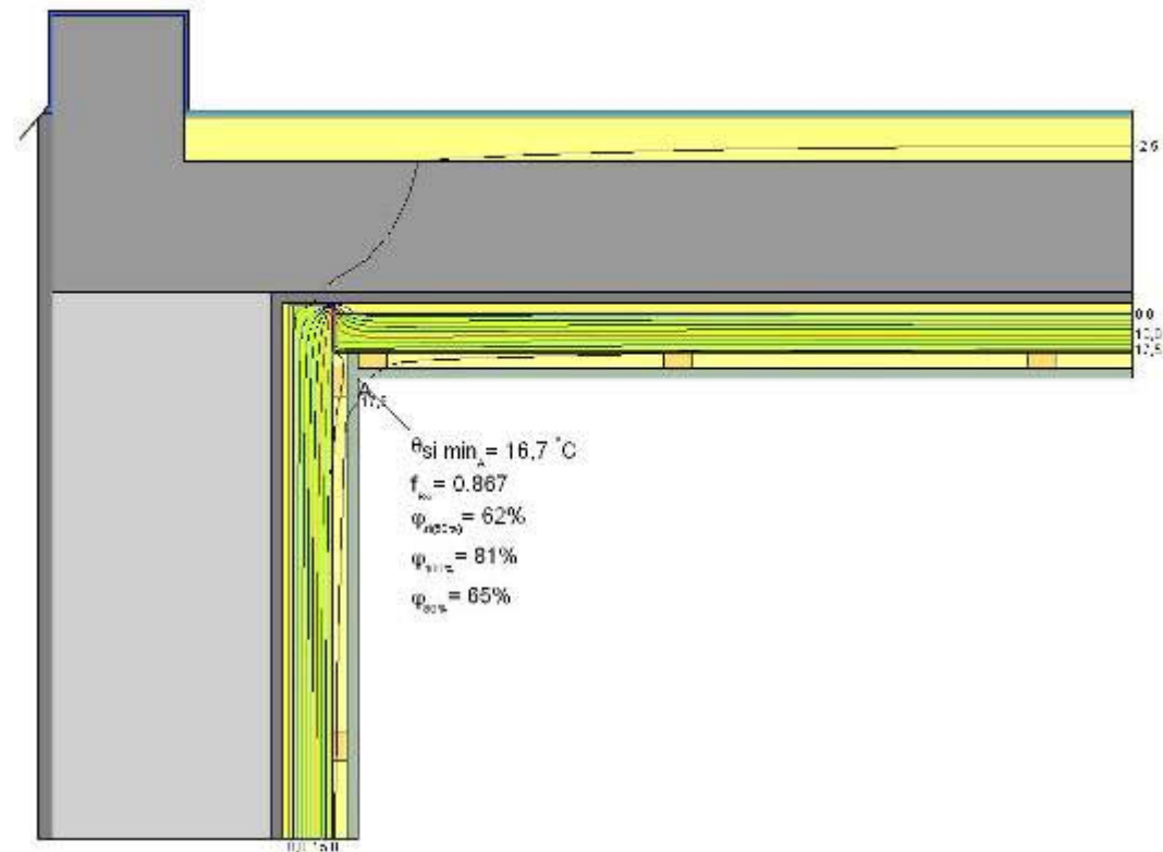
Detail 8; Temperaturen
