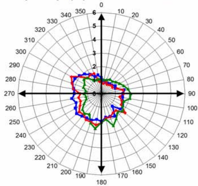
Anhang A 5: Polardiagramm Wind 3. Quartal 2008
