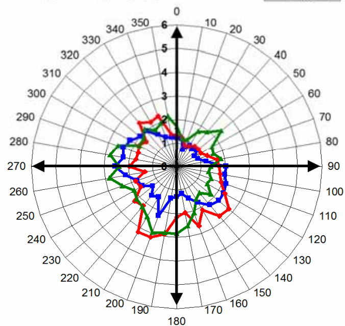
Anhang A 11: Polardiagramm Wind 1. Quartal 2010
