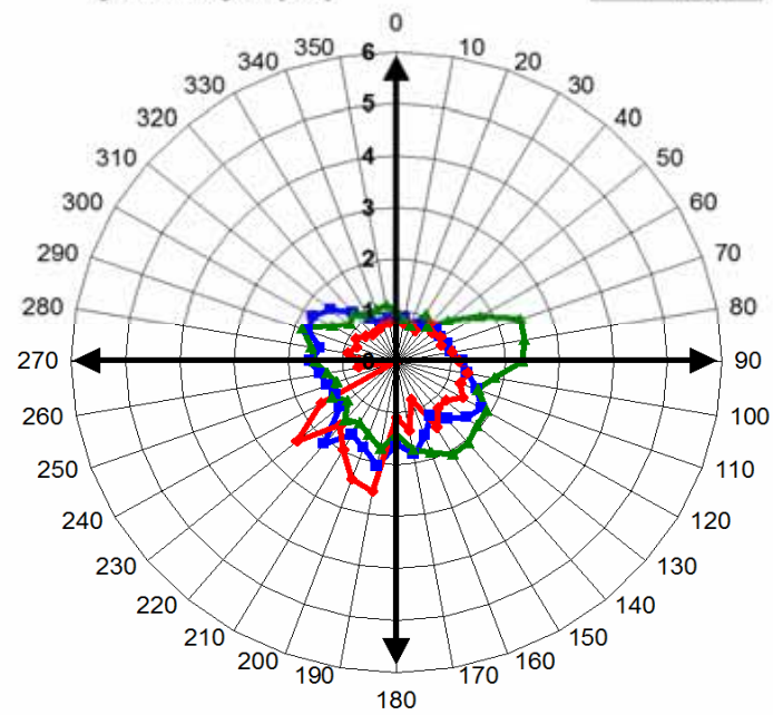
Anhang A 6: Polardiagramm Wind 4. Quartal 2008
