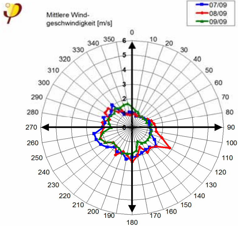
Anhang A 9: Polardiagramm Wind 3. Quartal 2009
