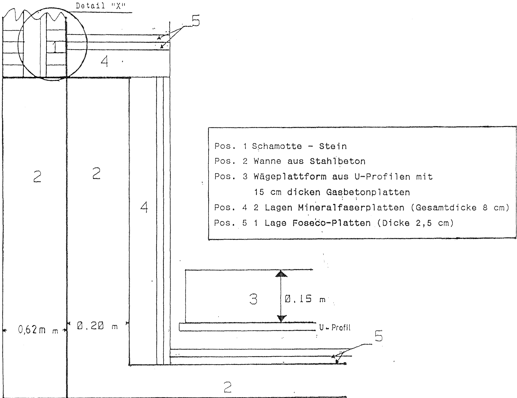
Abb. 4: Detail "A" zu Abb. 3
